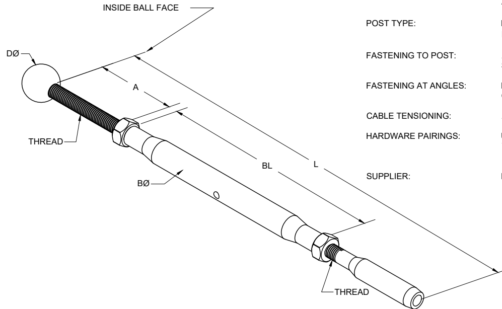
BALL END TURNBUCKLE, STAINLESS STEEL
