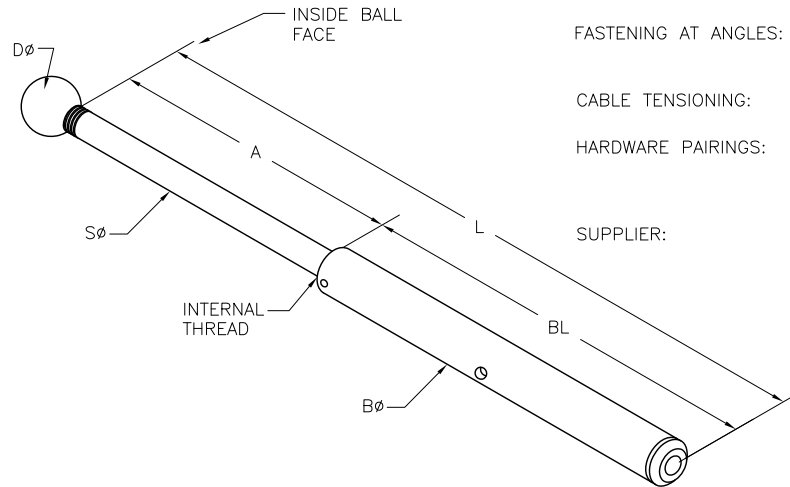
SLEEKLINE BALL END TURNBUCKLE, STAINLESS STEEL
