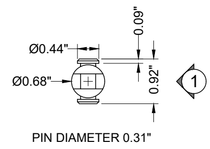
2 TENSION FORK - END VIEW SCALE = 1:2
