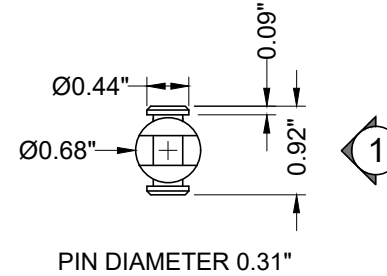
2 TENSION FORK - END VIEW SCALE = 1:2 PIN DIAMETER 0.31"
