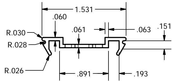
TOP VIEW SCALE 1 : 1
